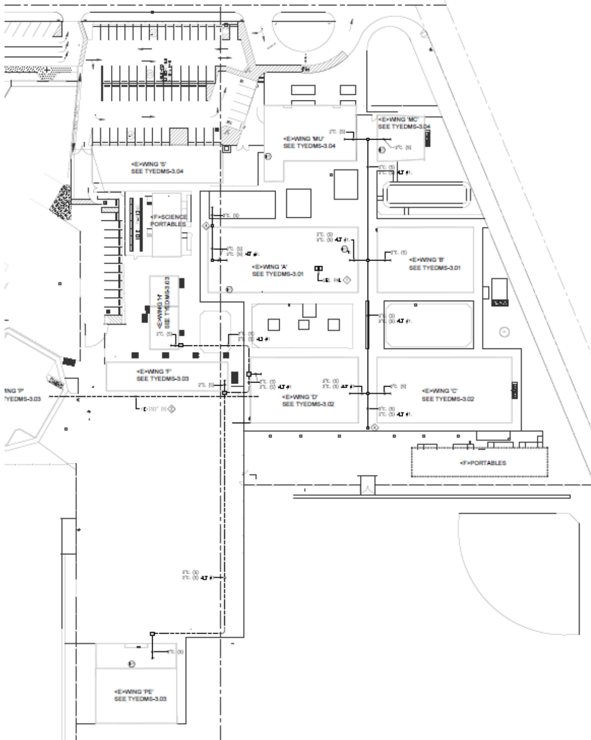
1 SITE PLAN
